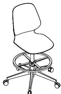
Extended-Height Seat Height 22¼-32¼"H Seat 17¾"W x 21¾"D Back 17"W x 16"H Overall 30½"W x 30½"D x 38-48"H
