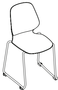
Stack (Sled Base) Seat Height 21"H Seat 17¾"W x 21¾"D Back 17"W x 16"H Overall 21¾"W x 21¾"D x 36½"H
