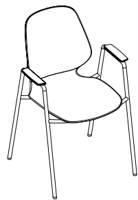
Guest Seat Height 19"H Seat 17¾"W x 21¾"D Back 17"W x 16"H Overall 23¼"W x 22¼"D x 34½"H
