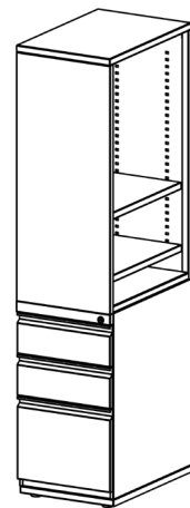
Bookcase Tower 15"W x 22.5" D x 56"H 15"W x 22.5" D x 65"H
