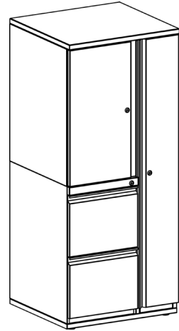
Cabinet Wardrobe Tower 24"W x 22.5" D x 56"H 24"W x 22.5" D x 65"H
